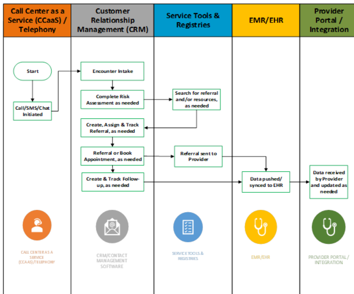
Figure 14 Call Process
