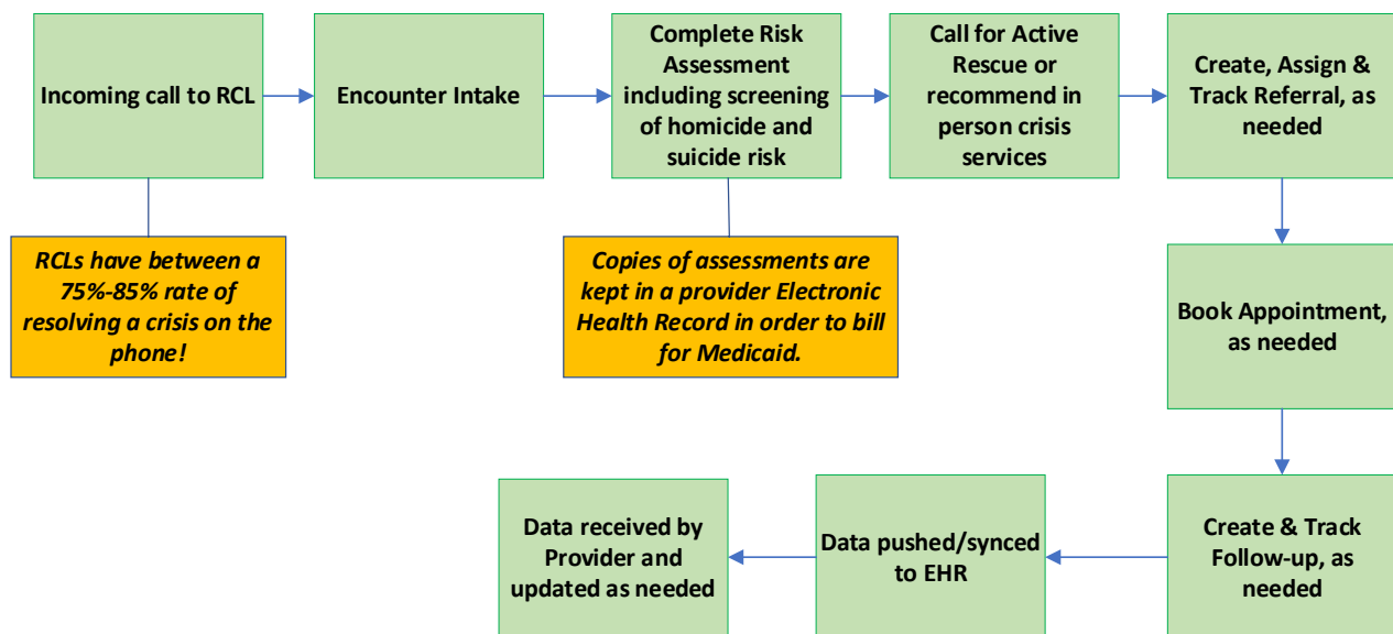
Figure 21 RCL Process
