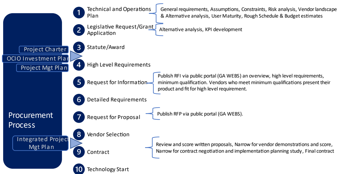
Figure 68 Procurement Process
